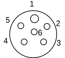
Impulse RMG-6-FS Female Face
