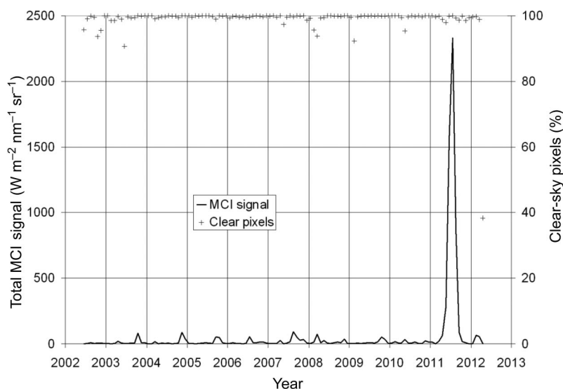
Figure 5. Monthly time series of MERIS MCI signal integrated over the rectangular area 5^{\circ} – 9^{\circ} N, 35^{\circ} – 50^{\circ} W. The high signal in July 2011 is about a factor 200 larger than any signal previously observed in July. The plot of clear sky pixels shows that 90% of months have better than 98% coverage, and only April 2012, for which MERIS provided only 4 days of data before ENVISAT failed, has less than 90%.
