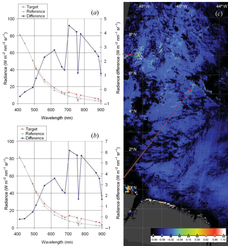
Figure 3. Spectra ((a) and (b)) and MCI 1.2 km resolution image (c) of floating vegetation north of the Amazon River mouth on 29 June 2011, showing the chlorophyll 'red edge' in slick spectra (red, positions indicated by red arrows, radiances measured at the satellite) and clearly visible in difference spectra (dark blue line, values on right-hand y-axis) after the reference spectrum (green) of nearby clear water is subtracted. Image colour sequence is as for Figure 2.
