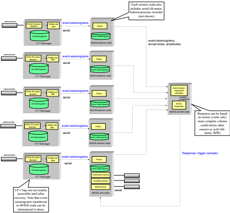
Axial Software Deployment Diagram (version 1.1)
