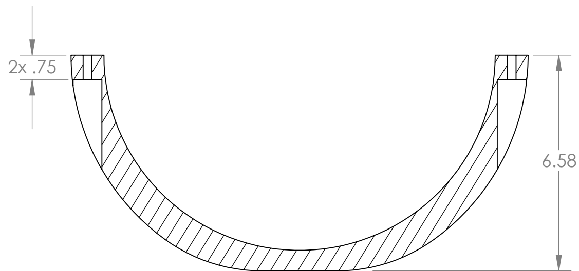
SECTION C-C SCALE 1 : 3
