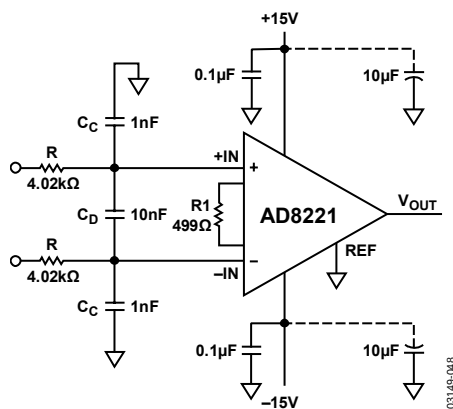
Figure 48. RFI Suppression
