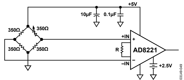
Figure 49. Precision Strain Gage
