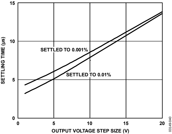
Figure 40. Settling Time vs. Step Size ( G = 1 )
