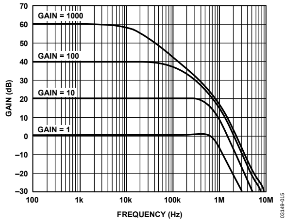
Figure 15. Gain vs. Frequency
