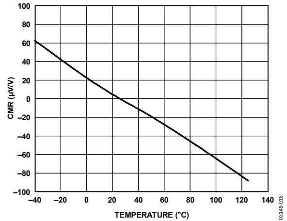
Figure 18. CMR vs. Temperature
