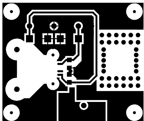
Figure 45. Bottom Layer of the AD8221-EVAL
