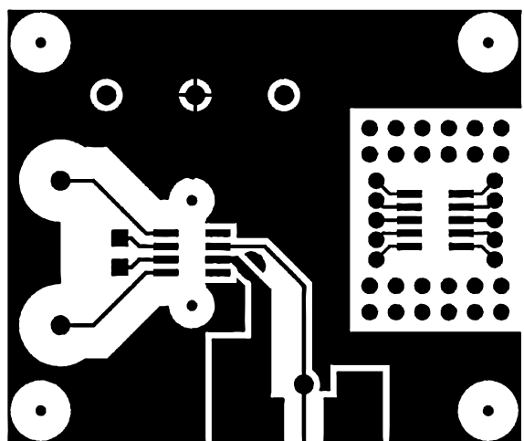
Figure 44. Top Layer of the AD8221-EVAL
