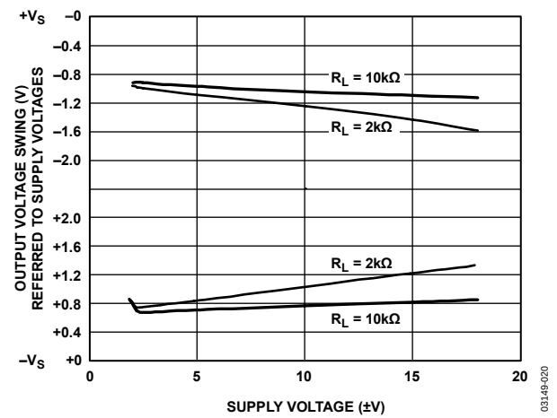
Figure 20. Output Voltage Swing vs. Supply Voltage, G = 1
