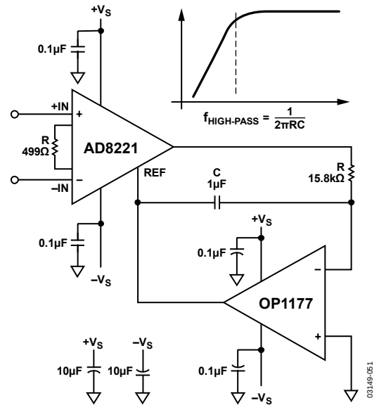
Figure 51. AC-Coupled Circuit
