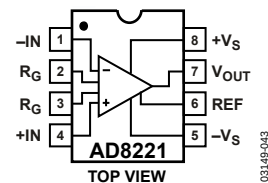
Figure 43. Pinout Diagram
