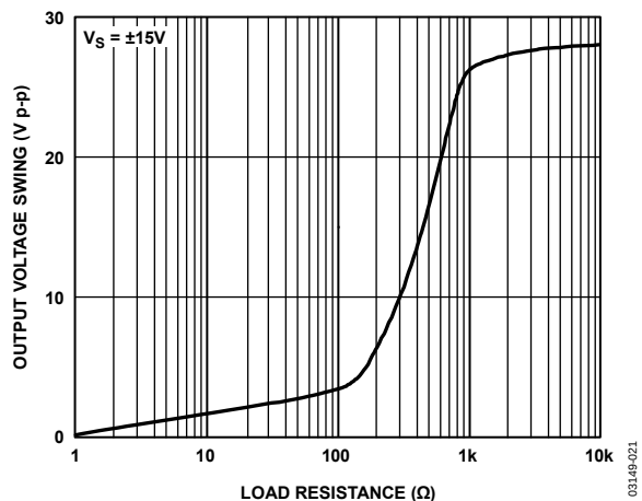
Figure 21. Output Voltage Swing vs. Load Resistance
