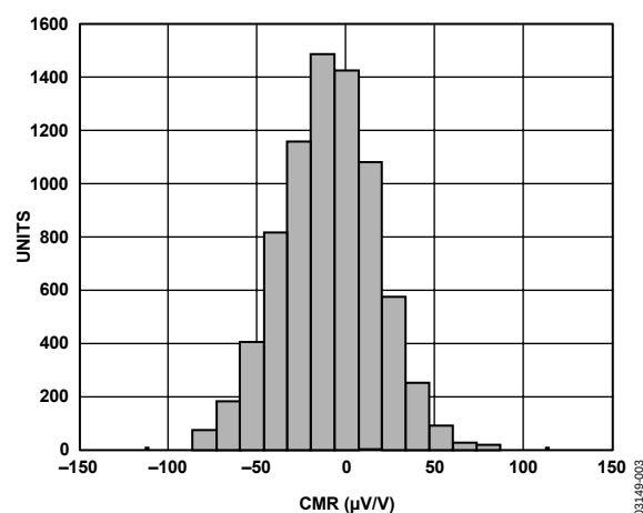
Figure 3. Typical Distribution for CMR ( G = 1 )
