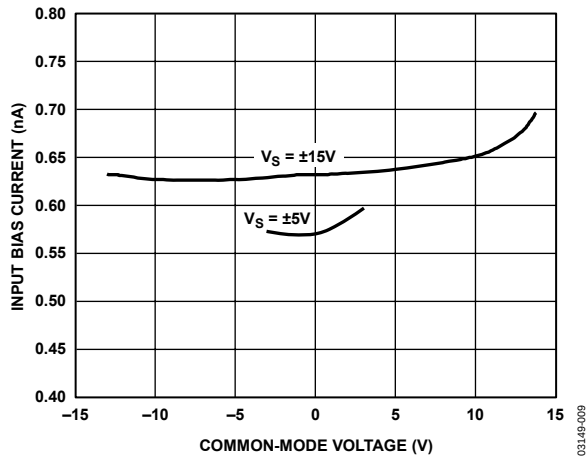
Figure 9. I_{BIAS} vs. CMV
