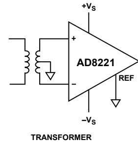
TRANSFORMER
