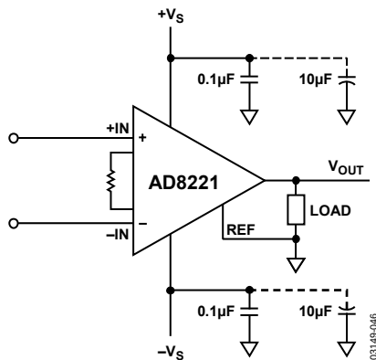
Figure 46. Supply Decoupling, REF, and Output Referred to Local Ground
