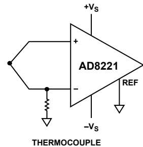
THERMOCOUPLE
