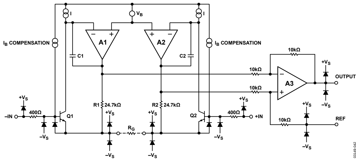
Figure 42. Simplified Schematic
