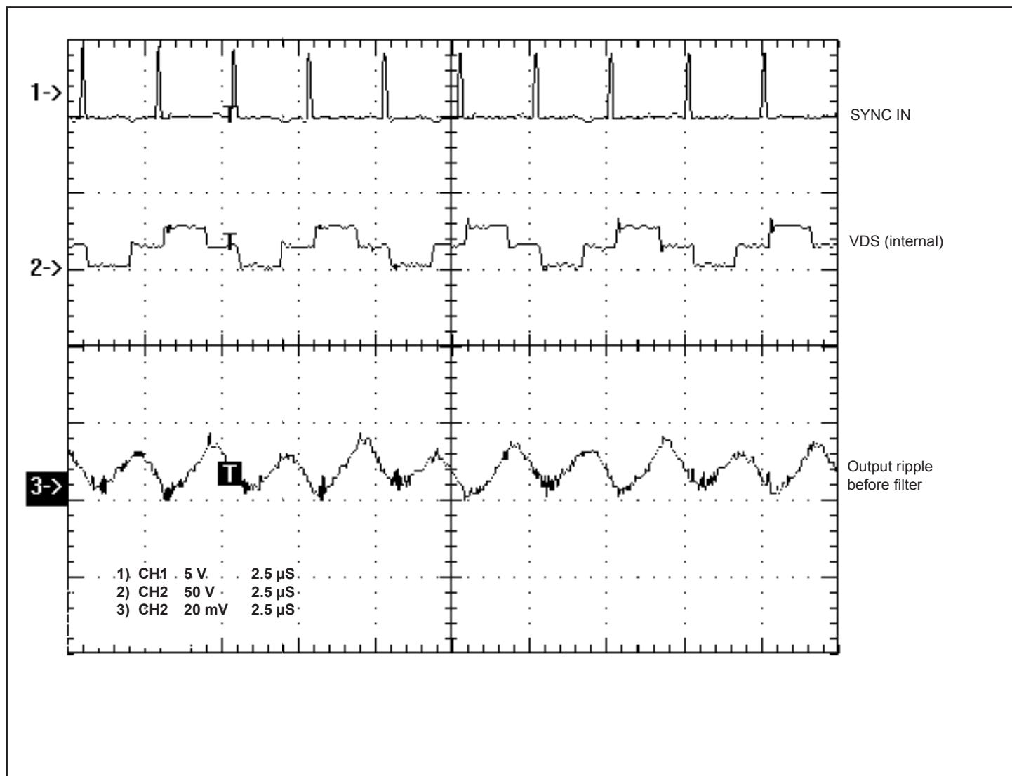
FIGURE 7. External Synchronization
