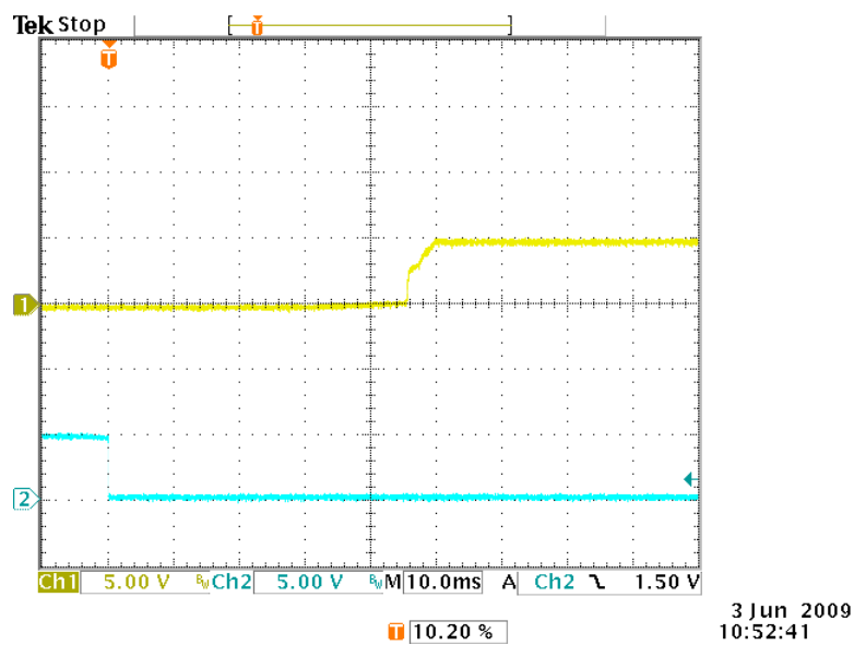
FIGURE 10. Output voltage delay and rise time at V_{in}=24 , I_{out}=5A using ON/OFF pin on the Q25S5/24.
