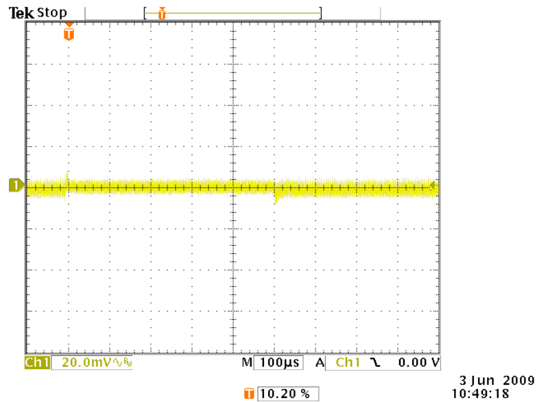
FIGURE 9. Transient Response at V_{in}=24 , I_{out} changing from Full load to Half load on a Q25S5/24.
