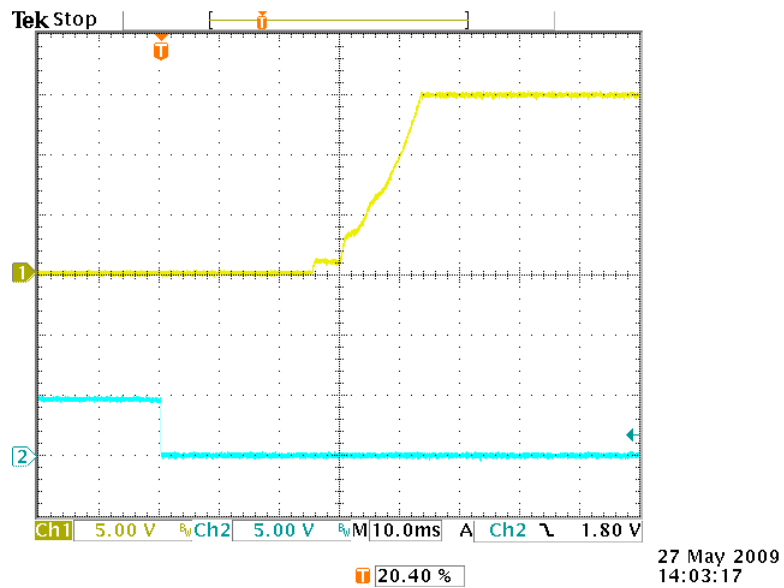
FIGURE 12. Output voltage delay and rise time at V_{in}=24 , I_{out} at Full load using ON/OFF pin on the Q25D15/24.
