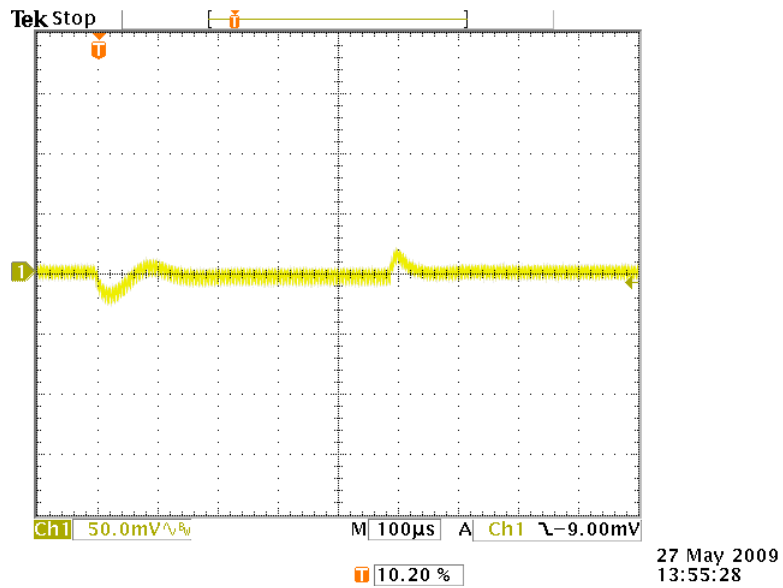
FIGURE 11. Transient Response at V_{in}=24 , I_{out} changing from Full load to Half load on a Q25D15/24.
