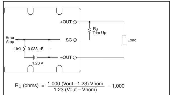
Figure 8 — Output voltage trim up circuit.
