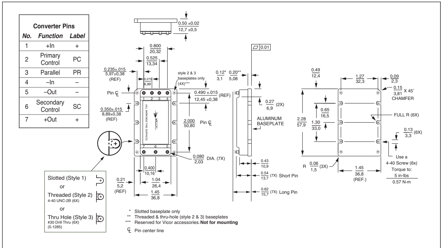
Figure 13 — Module outline
