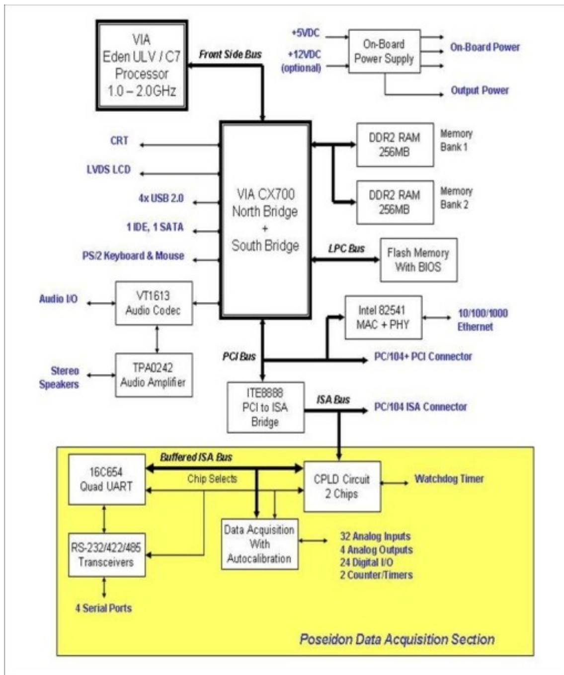
Figure 1: Poseidon Functional Block Diagram
