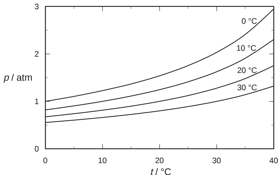
Figure 1. Pressure in head-space, with r = 0.01 , as a function of temperature for various initial temperatures. In calculating this, it was assumed that the gases \text{N}_2 , \text{O}_2 , Ar, \text{H}_2\text{O} were initially at solubility equilibrium with sea water at the starting temperature, that they behaved ideally and that the initial pressure in the bottle at the indicated temperature was 1 atm.
