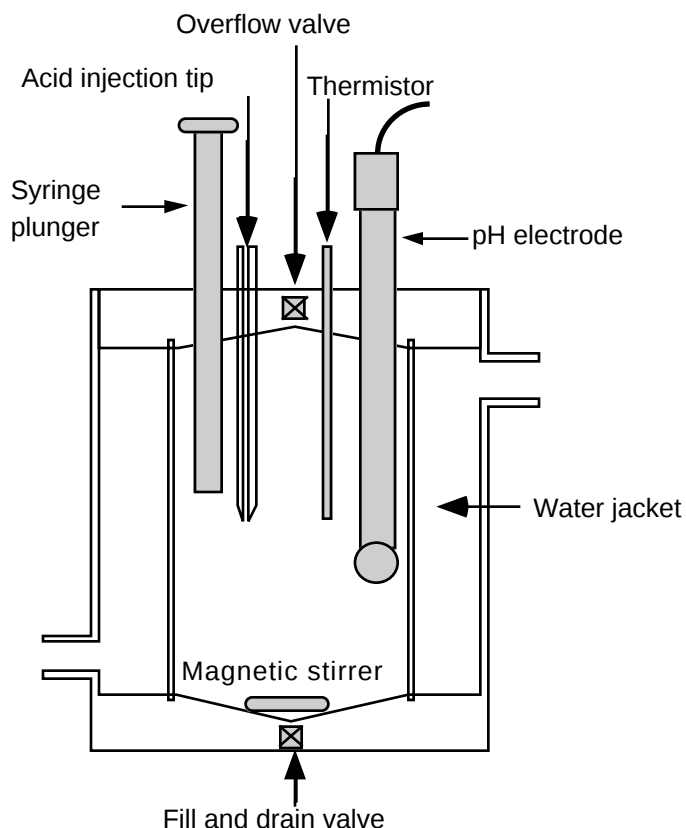
Figure 1. Closed titration cell for the determination of alkalinity.
