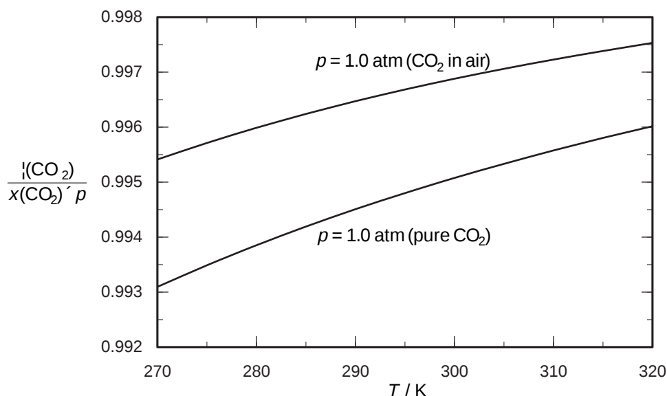
Figure 1. Variation of fugacity coefficient with temperature at 1 atm total pressure for pure \text{CO}_2 gas and for \text{CO}_2 in air: x(\text{CO}_2) = 350 \cdot 10^{-6} (calculated using the procedure described in SOP 24 of this Handbook).
