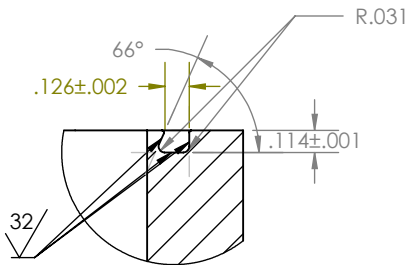
Half-Dovetail Groove for 1/8" Dia. O-ring DETAIL D
