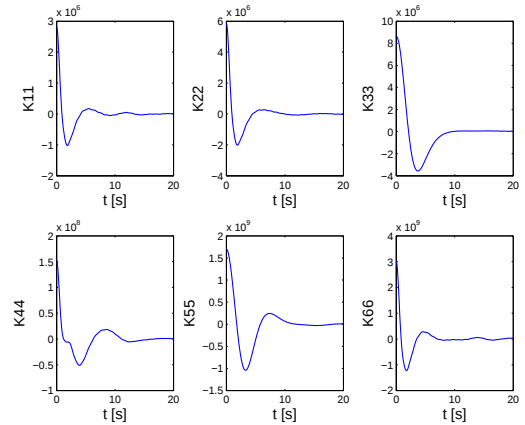
Fig. 8. Retardation functions for a symmetric barge 8x45m at zero speed.
