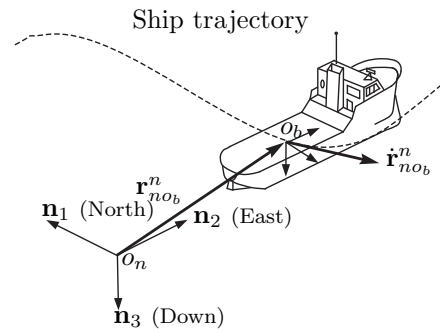
Fig. 4. Ship position and velocity vectors.
