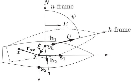
Fig. 5. Seakeeping coordinates. In absence of wave excitation, the frames h - and s -frame coincide.
