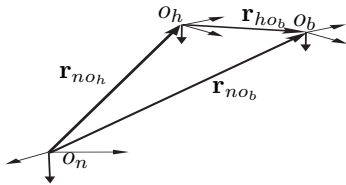
Fig. A.1. Relative position of frames.
