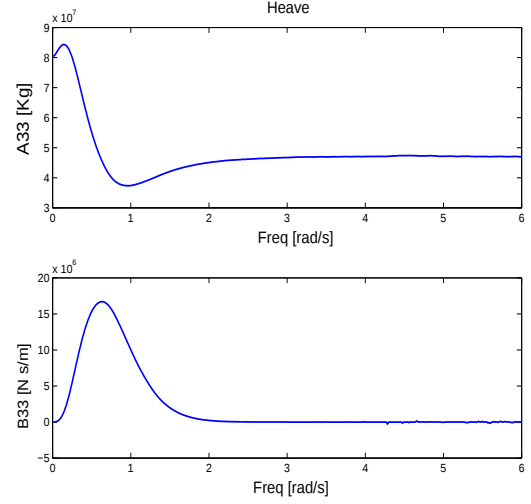
Fig. 6. Heave added mass and potential damping for a symmetric barge 8x45m at zero speed.
