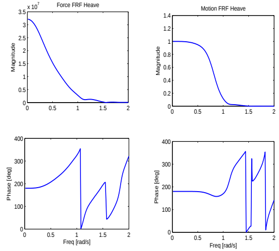
Fig. 7. Force and Motion FRF in for a symmetric barge 8x45m at zero speed.
