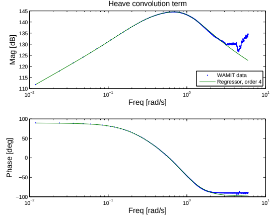
Fig. 10. Convolution term FRF K_{33}^h(\omega) and its estimate \hat{K}_{33}^h(\omega) .
