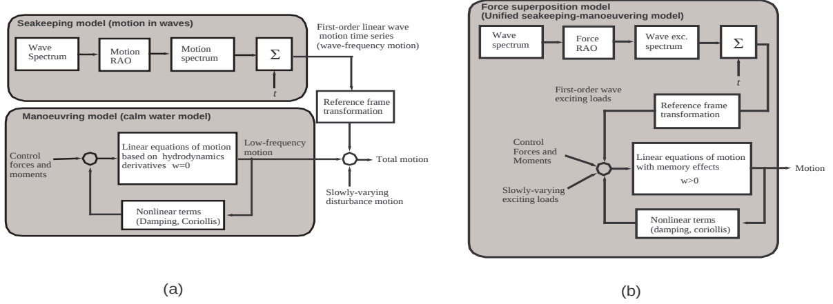
Fig. 3. Models of marine vessels for control. (a)-motion superposition model; (b)-force superposition or unified model.
