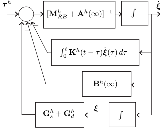
Fig. 9. Block diagram representation of the Cummins Equation
