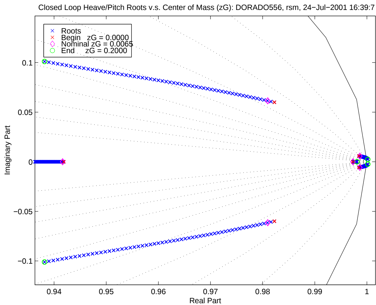
Figure 13: Partial Root Locus of the Depth Control System on Center-of-Mass
