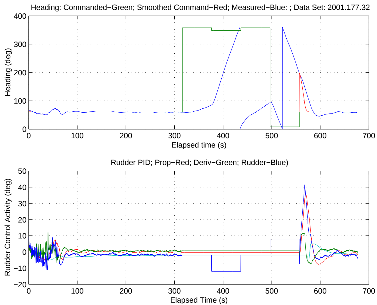
Figure 15: Heading and Rudder Angles
