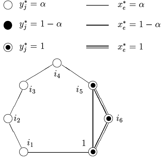
Figure 2.1: Fractional point violating a cycle cover inequality for the OP instance with t_0=6 and t_e=1 for all e \in E ( 0 < \alpha \leq 1/2 ). Here T = \{[1, i_1], [i_1, i_2], \dots, [i_6, 1]\} , x(T) = 2 + 5\alpha , and y(V(T)) = 3 + 4\alpha .
