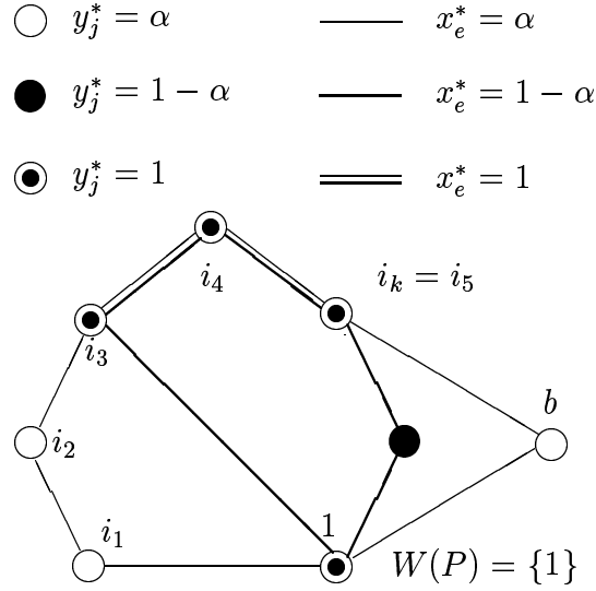
Figure 2.2: A fractional point violating a path inequality for the OP instance with t_0=6 and t_e=1 for all e \in E ( 0 < \alpha \leq 1/2 ).
