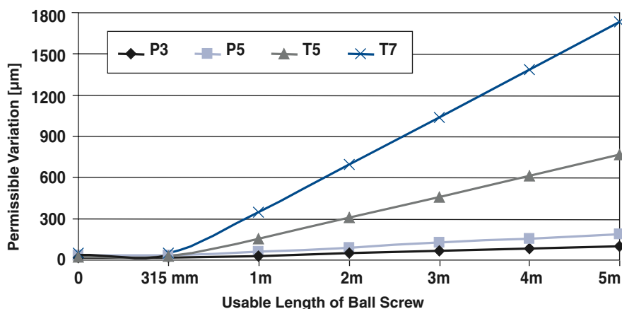
Cumulative Lead Variation Over Usable Length
