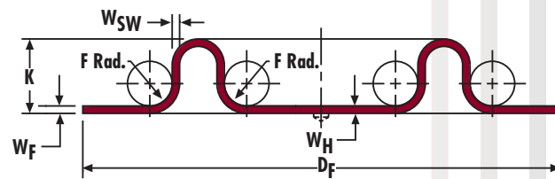
Fig. 10: Preconvoluted Diaphragm
