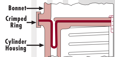
Fig. 21: Crimp-Ring Design
