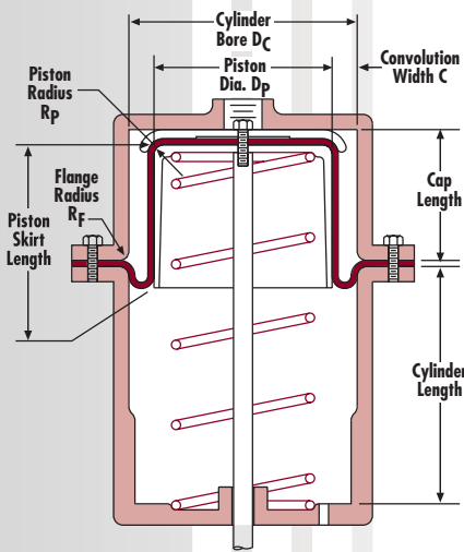
Fig. 17: Hardware Dimensions
