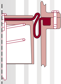
Fig. 18: Diaphragm inversion resulting from lack of curved retainer plate.
