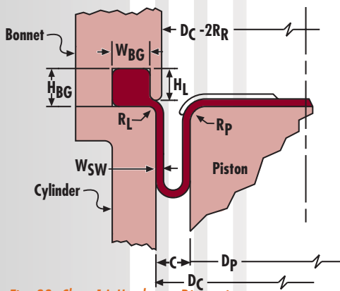
Fig. 28: Class 1A Hardware Dimensions
