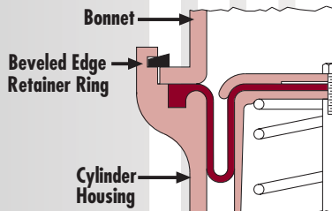
Fig. 27: Beveled Edge Retainer Plate
