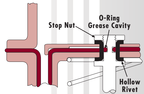
Fig. 39: Slip Joint Shaft Assembly
