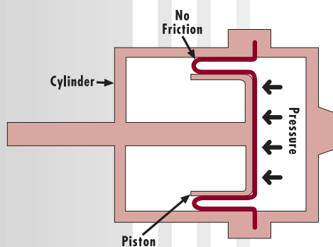
Fig. 1: Rolling Diaphragm installed in cylinder
