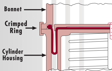
Fig. 29: Crimped Ring
