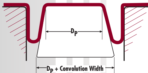
Fig. 40: Tapering the Piston
