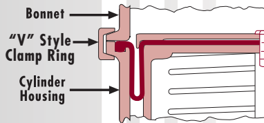
Fig. 25: Ring Clamp
