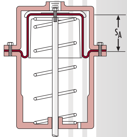
Fig. 7: Up-Stroke Position
