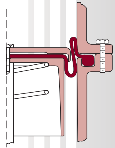
Fig. 38: Pressure Reversal of Diaphragm
