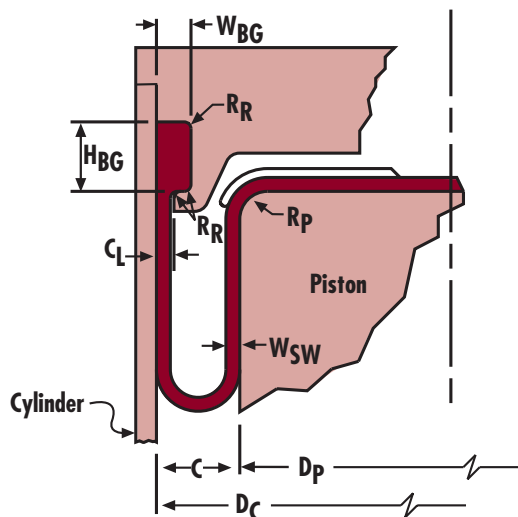
Fig. 33: Radial Compression (note 1) with Cast Machined Retainer Plate
