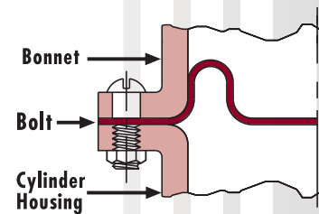
Fig. 23: Bolted Flange
