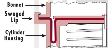
Fig. 22: Swaged Lip
