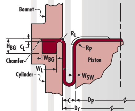
Fig. 24: Classes 3 and 3C Hardware Dimensions
