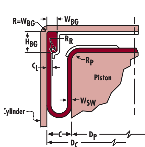
Fig. 32: Axial Compression with Stamped Retainer Plate
