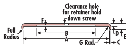
Fig. 20: Curved lip retainer for Classes 3, 4, 1A and 1B ("Top-Hat" Diaphragms).
