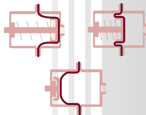
Fig. 13: Involute Diaphragm cycle. Convolution is not required at stroke limits.
