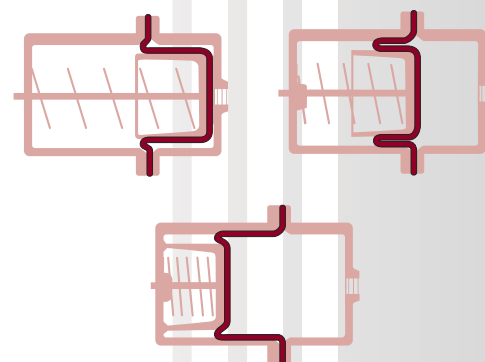
Fig. 12: Standard rolling diaphragm cycle. Convolution is present at all times.
