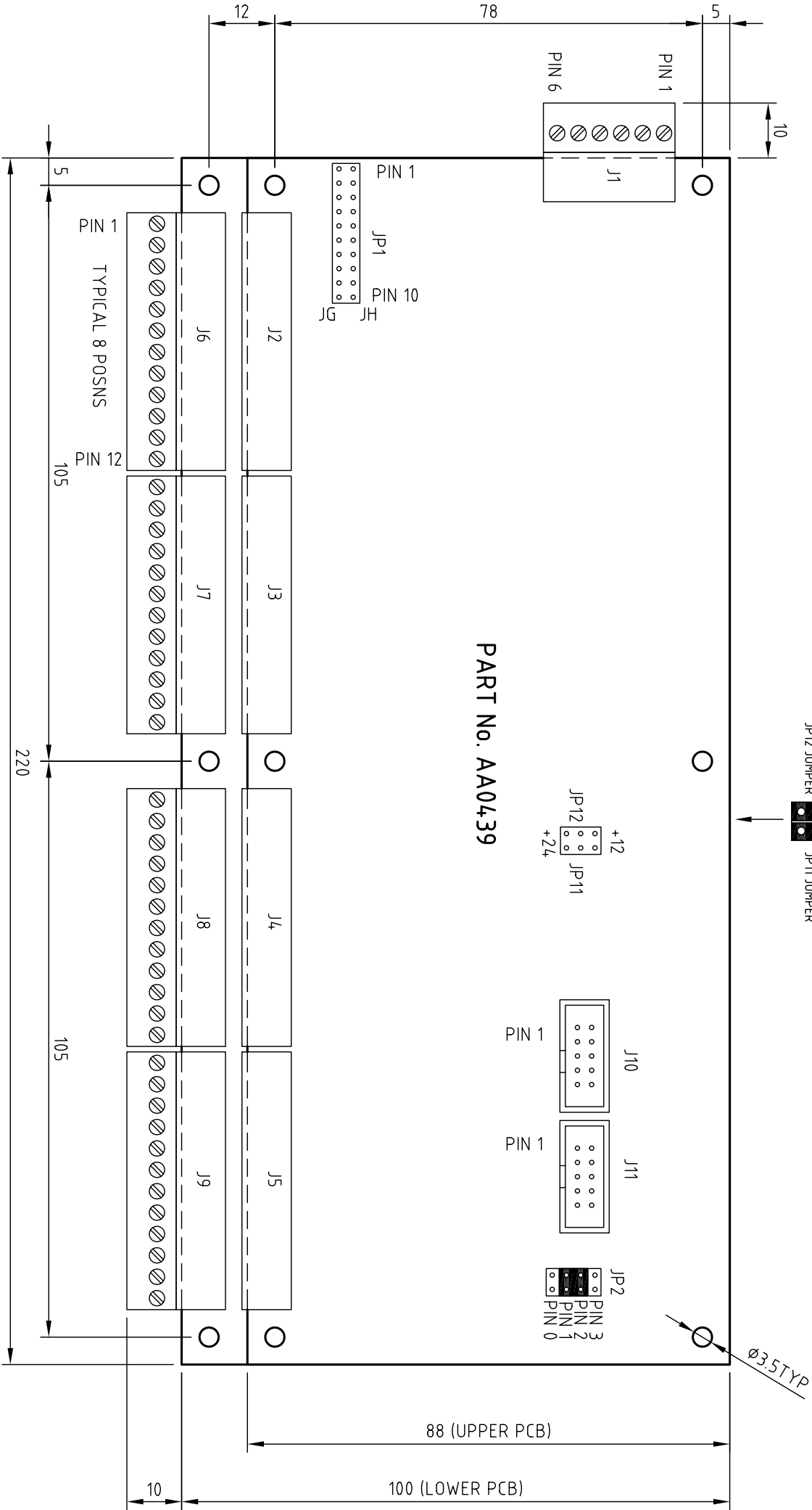
PLAN VIEW ON DOUBLE PCB ASSEMBLY SCALE 1:1
