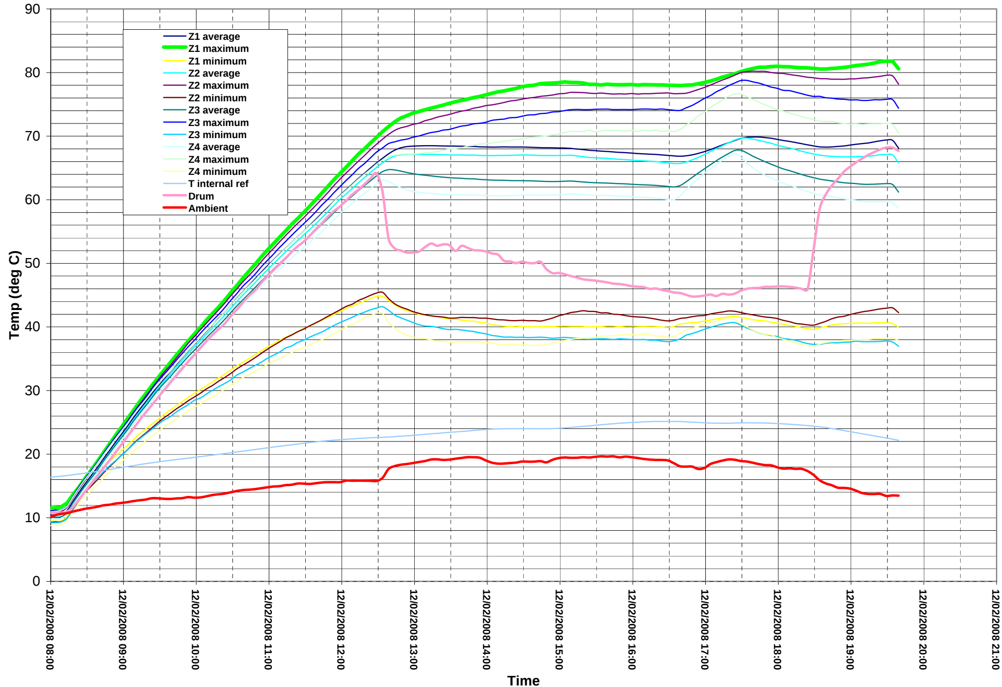
MBARI Umbilical Test @ 14.8A (12th Feb 2008)
