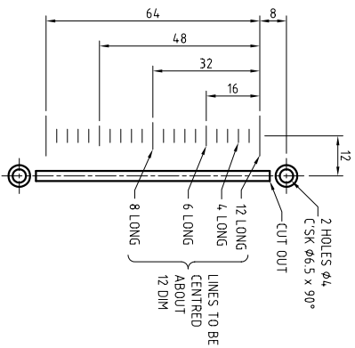
DETAIL 'B' (TYPICAL 3 PLACES)
