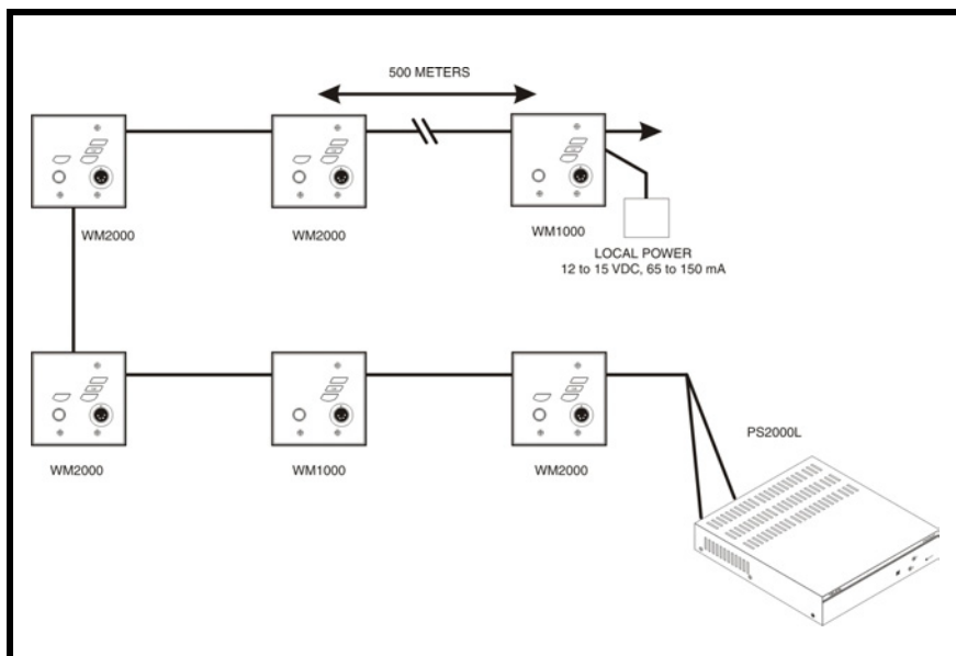
FIGURE 2. A two-channel intercom system using a PS2000L Power Supply set to isolate mode. In isolate mode, each intercom channel is a separate party line, and total current for each channel is limited to 1 amp. Note, both WM1000 and WM2000 stations may be connected, depending on each locations need to communicate with one or two channels. WM1000 stations may be connected to either channel one or two. Also note, locally powered stations may be connected. This is recommended when stations are installed at remote locations. Since the PS2000L provides termination for the intercom channels, no user-installed termination is required. For WM1000 connection details, refer to Figure 6, for WM2000, refer to Figure 7.
