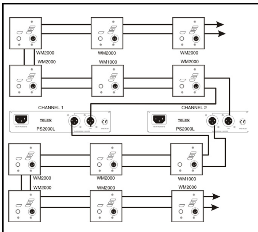
FIGURE 4. A two-channel intercom system using two PS2000L power supplies. Each PS2000L is set to combine mode and it supplies power to one intercom channel only. Each intercom channel is a separate party line, and total current for each channel is limited to 2 amps. Note, both WM1000 and WM2000 Intercom Stations may be connected, depending on each locations need to communicate with one or two intercom channels. For WM1000 connection details, refer to Figure 6, for the WM2000 refer to Figure 7.
