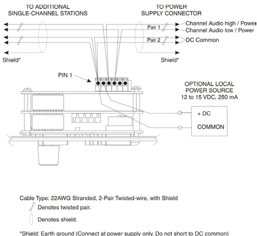
FIGURE 6. Audiocom mode connections for WM1000 Intercom Station.
