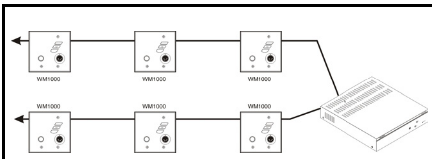
FIGURE 3. A single-channel intercom system using one PS2000L with WM1000 Intercom Stations. The PS2000L may be set to either combine or isolate mode. In combine mode, all intercom stations talk on a single party line, and total current for the channel is 2 amps. In isolate mode, one string of intercom stations is operated as channel one, and the other string is operated at channel two. There is no communication between the separate channels, and the total current per channel is 1 amp. For WM1000 connection details, refer to Figure 6.
