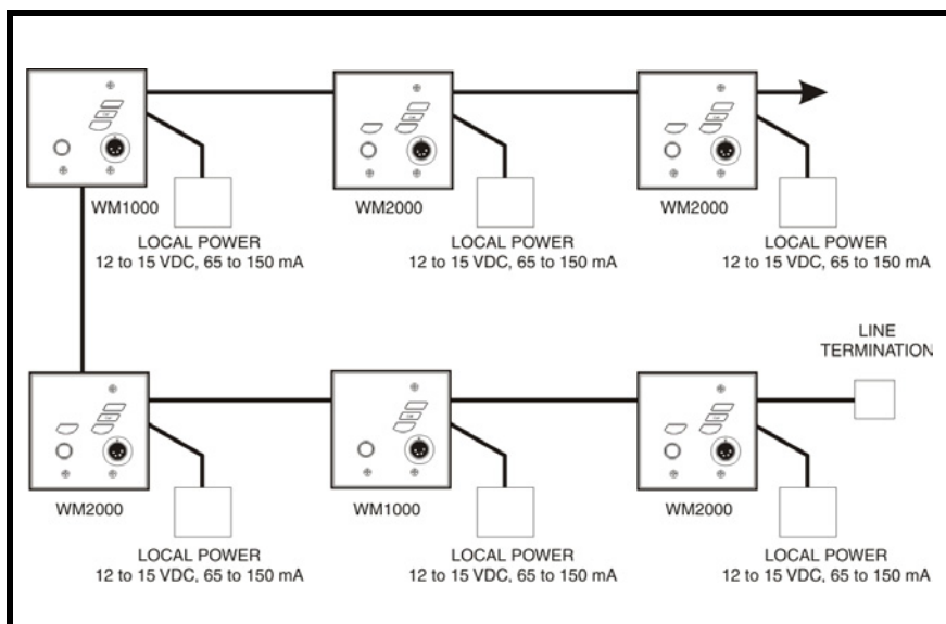
FIGURE 5. An example of an intercom system using all local powered stations, with no power being distributed on the intercom channels (dry lines). WM2000 stations are shown, but WM1000 stations by also be used. Since an Audiocom power is not used, the install must connect a line termination somewhere in each channel for proper operation. The required line termination is shown in Figure 8.
