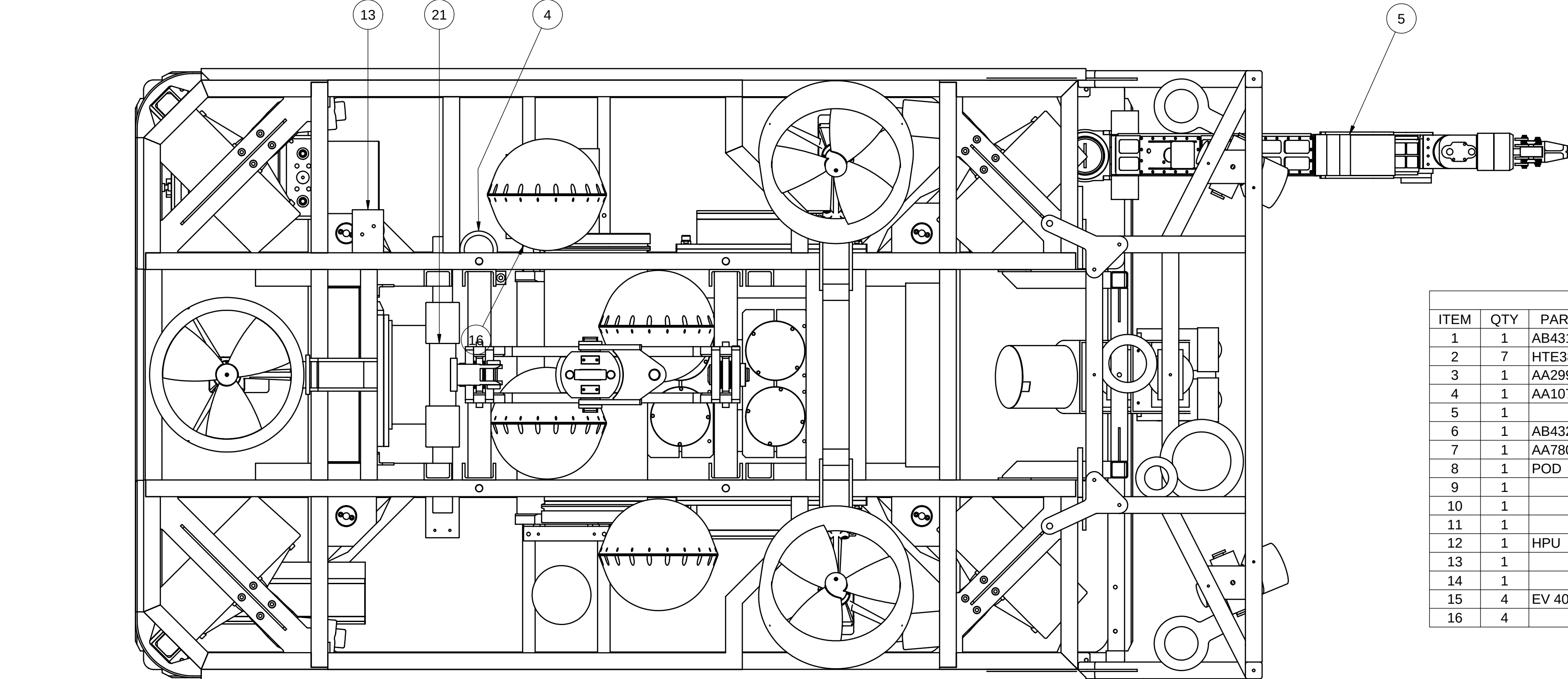
PLAN VIEW (NO BUOYANCY)
