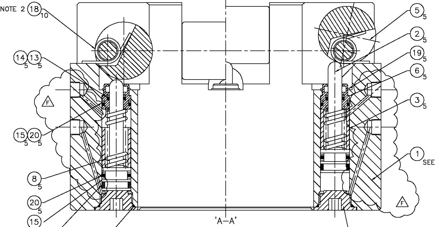
LATCH ROLLER IN THE 'LATCHED' POSITION
