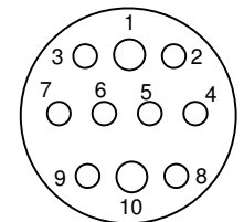
MINK-10-CCPL PINS, FACE VIEW
