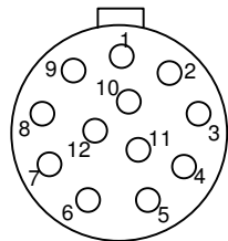
1041031 PINS, FACE VIEW
