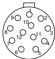
1041031 PINS, FACE VIEW
