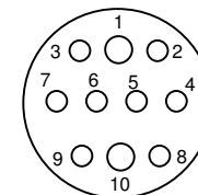
MINK-10-CCPL PINS, FACE VIEW
