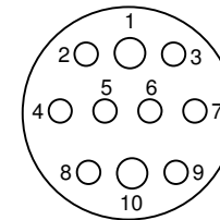
MINK-10-CCRL SOCKETS, FACE VIEW
