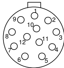
1041031 PINS, FACE VIEW
