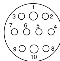
MINK-10-CCPL PINS, FACE VIEW
