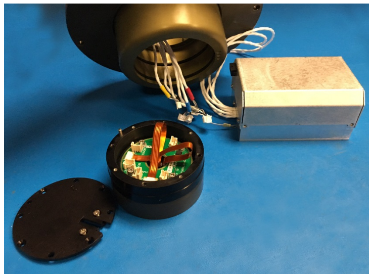
OEM Pathfinder Transducer Connections
