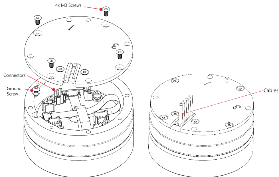
OEM Pathfinder Transducer Connections
