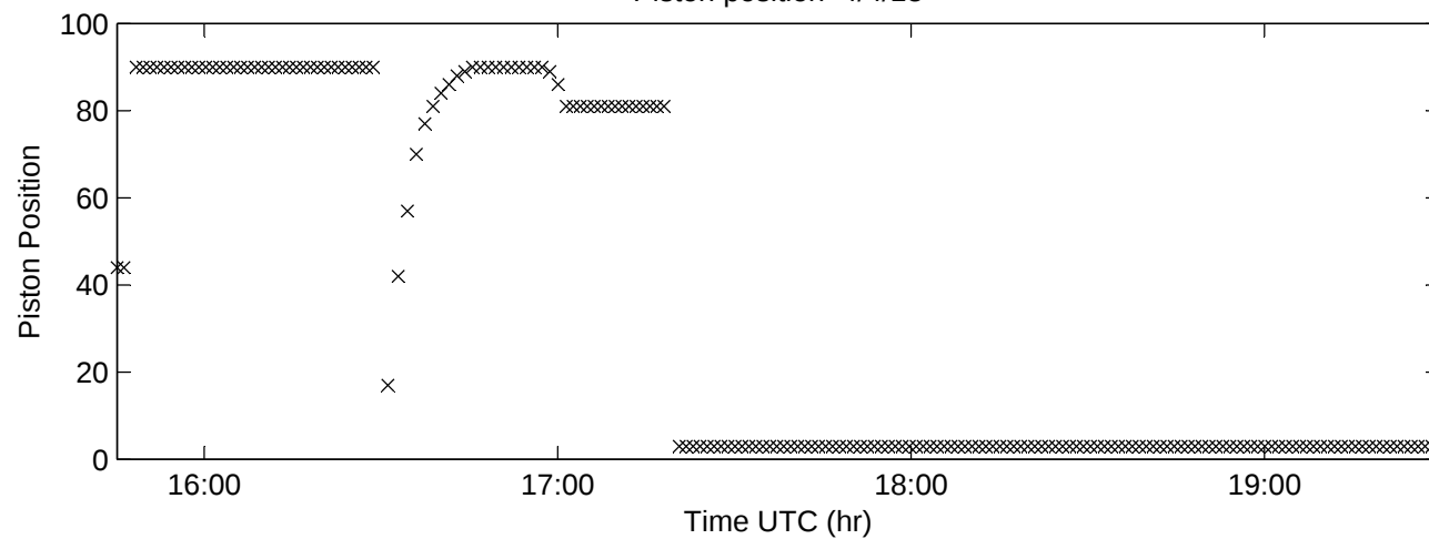
Piston position 4/4/13
