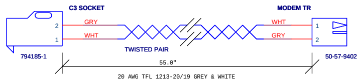
MODEM CABLE
