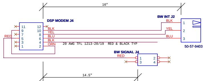
MODEM TO BURNWIRE INTERFACE CABLE
