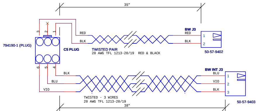
BURNWIRE INTERFACE CABLE
