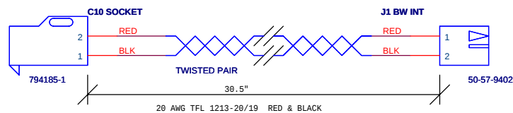
BURNWIRE INTERFACE POWER
