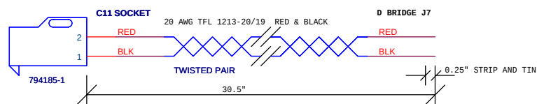
BURNWIRE INTERFACE POWER
