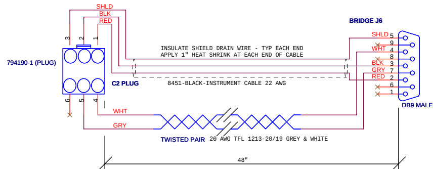
CONFIGURATION PORT CABLE
