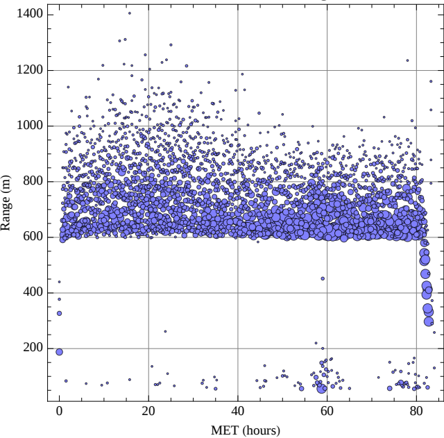
LST3 Dive 1 Sonar Ranges
