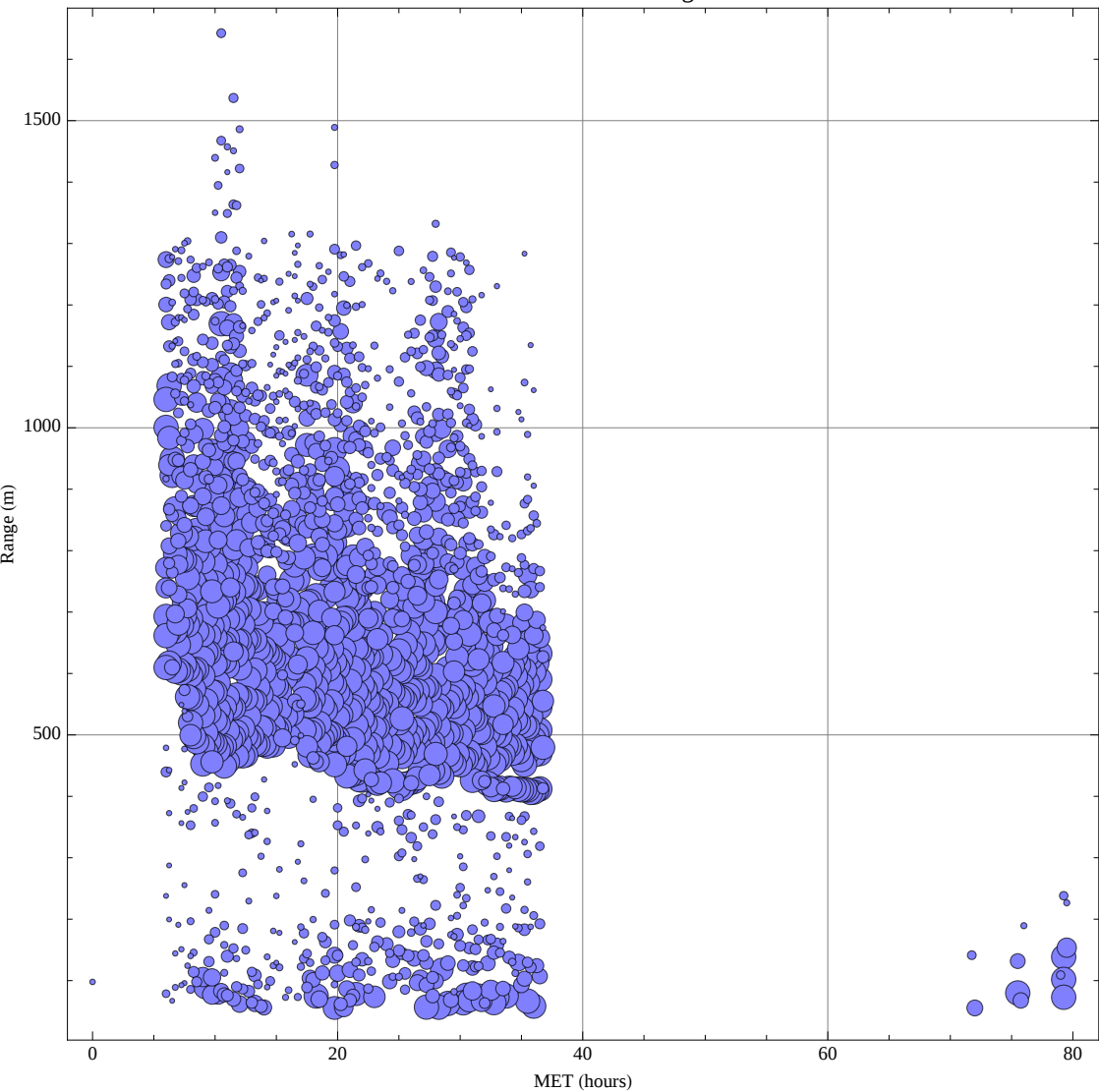
LST Dive 2 Sonar Ranges
