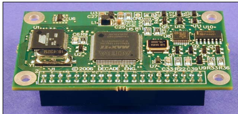
BOB-4-H (2x20 header format)
