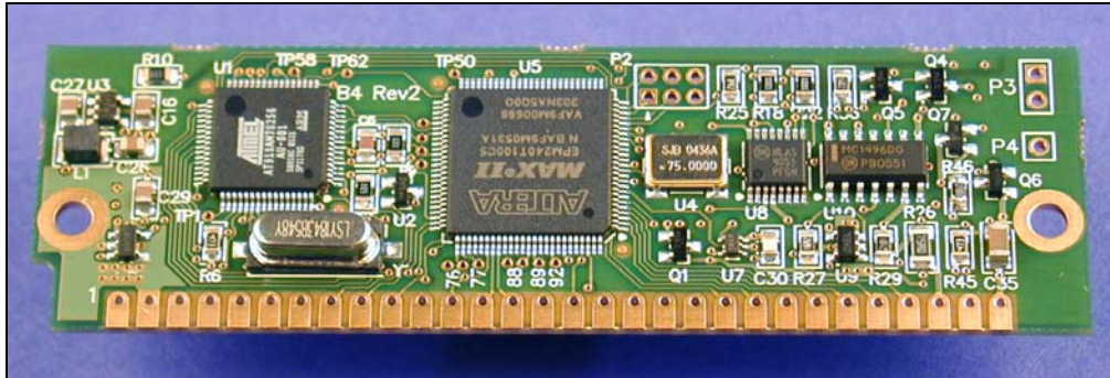
BOB-4-S (30-pin SIMM format)
