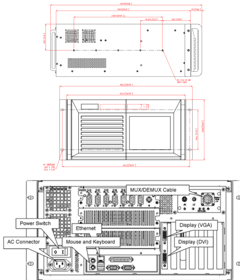
7-P Sonar Processor Unit (Rear Panel)
