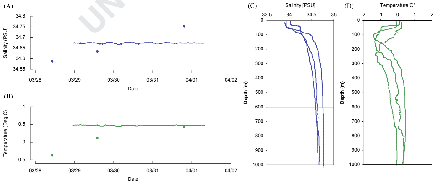
Fig. 4. The salinity (A) and temperature (B) measurements taken with the LST (line) and those taken from ship-based CTD casts (dots) at the same depth over the same time period. Vertical profiles of salinity (C) and temperature (D) taken from three CTD casts. The distances between the LST drop site and the three ship-based CTD casts were 22.2 km (March 28), 18.8 km (March 29), and 21.7 km (March 31).
