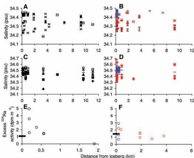
Fig. 2. Surface salinity and excess ^{224}\text{Ra} measured with increasing distance from icebergs W-86 and A-52. Black symbols represent measurements around W-86. The first and second sampling periods around A-52 are differentiated by blue and red symbols, respectively. (A and B) Mean surface salinity ( \pm \text{SE} ) at meter increments between 0 and 10 m depth determined from CTD casts [open squares; n = 10 measurements (W-86), n = 13 measurements (A-52)] and underway flow system salinity (intake at 5 m depth) determined at 1-min intervals for 5 min [crosses; n = 79 measurements (W-86), n = 100 measurements (A-52)]. The SE of each mean value is generally smaller than the representative symbol. (C and D) Mean salinity ( \pm \text{SE} ) determined from 10 CTD casts at W-86 and 13 casts at A-52 over the following depth intervals: 0 to 10 m (solid diamonds), 11 to 50 m (solid squares), 51 to 100 m (solid triangles), 101 to 200 m (dashes), 201 to 300 m (plus symbols), 301 to 400 m (“x” symbols), and 401 to 500 m (open circles). The SE for each mean value of each depth bin is generally smaller than the size of the representative symbol. (E and F) Excess ^{224}\text{Ra} in surface waters (0 to 10 m depth) with increasing distance from icebergs W-86 and A-52. The first sampling around A-52 (blue symbols) was more variable than the second sampling (red symbols), but the combined trends are similar. For comparison, nearshore sample activities ( <10 \text{ km} from the coastline of the Antarctic Peninsula; n = 7 measurements) are indicated by the black bar on the y axis. Average open ocean ( \geq 100 \text{ km} from any coastline in the Drake Passage; n = 6 measurements) and mixed-layer samples (30 to 80 m depth proximal to W-86 and A-52; n = 12 measurements) were at or below our detection limit of 0.6 \text{ dpm m}^{-3} , as was the zero value for W-86 (18). [The detection limit was calculated as three ( 3\sigma ) times our calculated counting error of 0.2 \text{ dpm m}^{-3} . The error was determined with Poisson statistics on the total counts for each counting interval and propagated based on three counting intervals per sample.]
