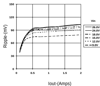
Ripple vs Output Current
