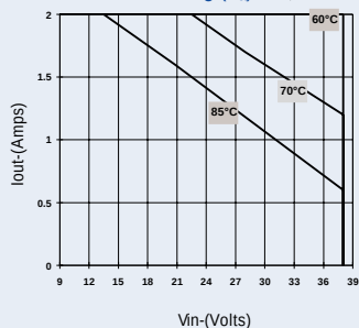
Thermal Derating ( T_a ) (See Note B)
