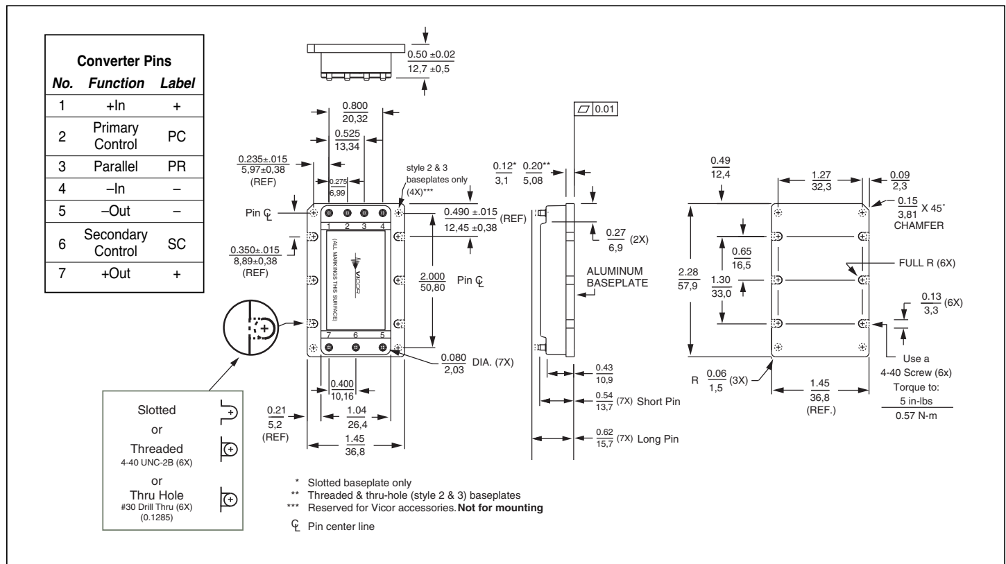
Figure 13 — Module outline
