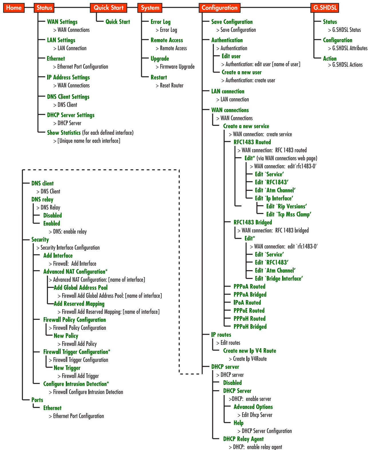
Figure 6. Model 3201/3241 Menu Structure
