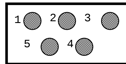
MALE PIN LPIL5M
