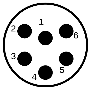
Subconn MCIL6F Face View
