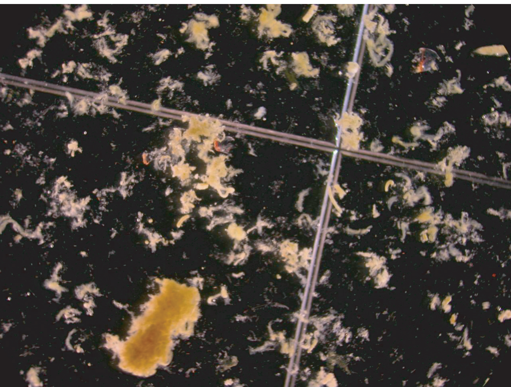
Detritus collected from Deployment 2: (Underneath C18A) Fecal pellets and exuviae collected under the influence of the iceberg.
