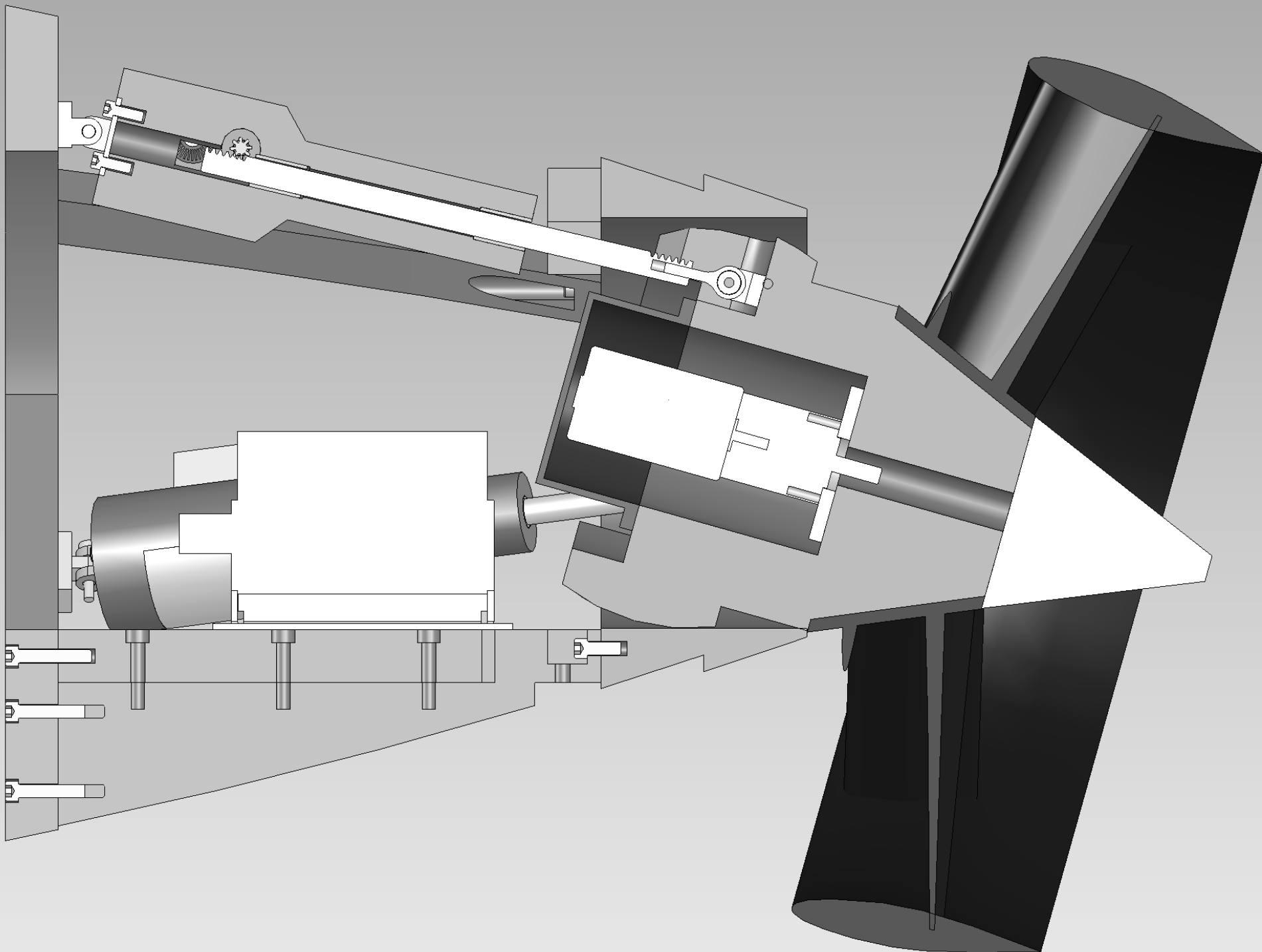
3 Actuator Tailcone - Normal Operation: Max Pitch Down
