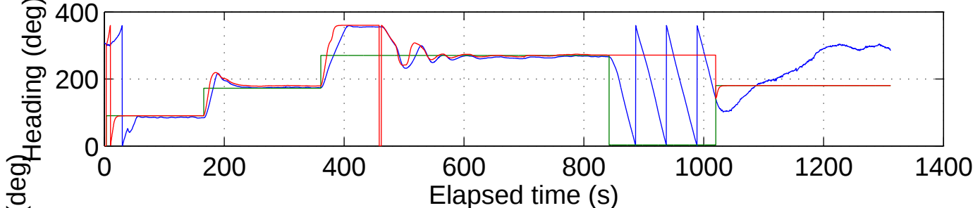
Rudder PID; Prop-Red; Deriv-Green; Rudder-Blue)
