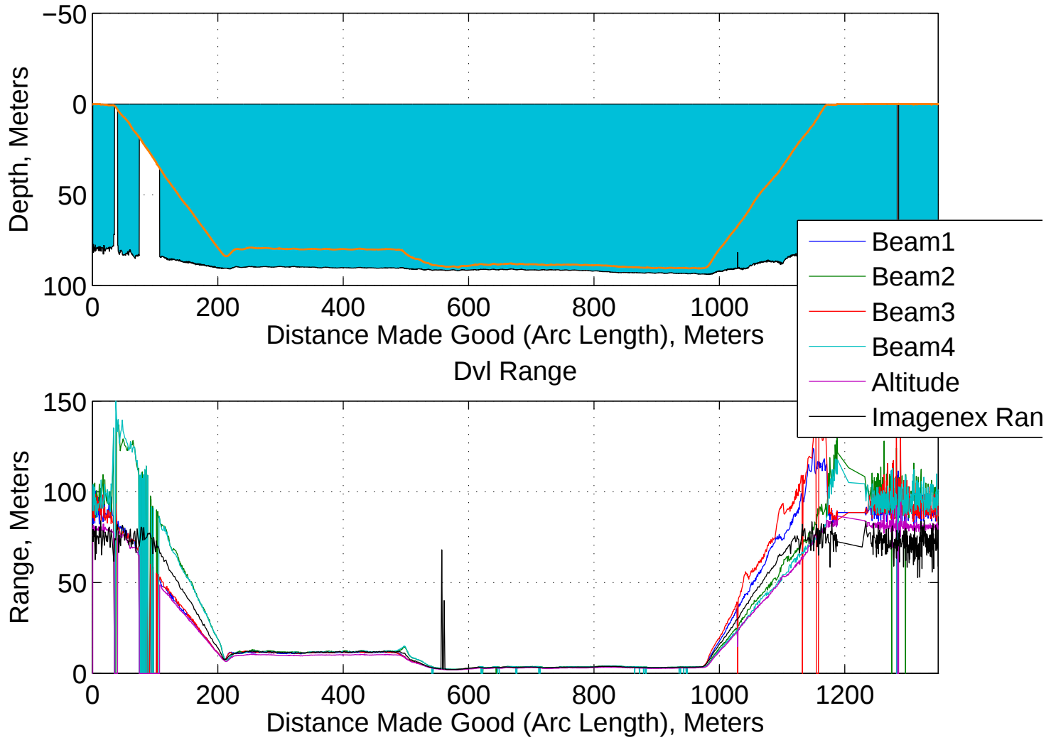
Vehicle and Bottom Depth: Data Set: 2009.293.11
