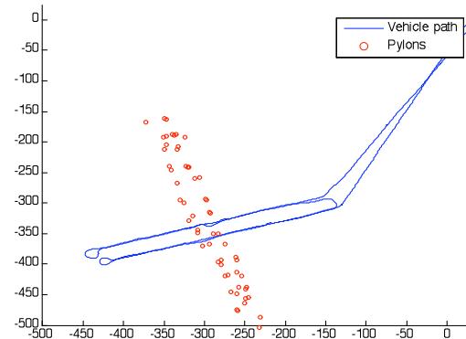
Figure 11. AUV trajectory with annotated positions of bridge pylons
