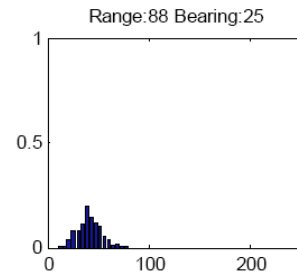
Figure 9c. Noise Histogram for the horizontal FLS at Range 88m and 25 degrees bearing
