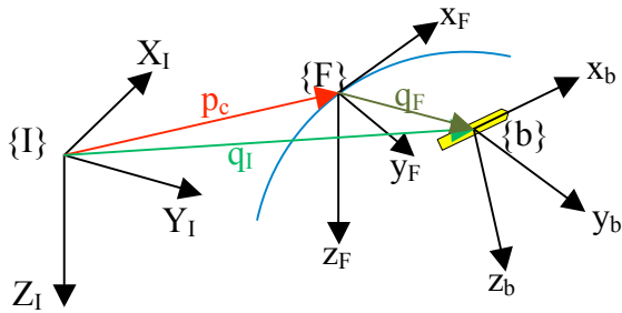
Figure 15. The inertial {I} frame, Serret-Frenet {F} error frame and the body-fixed reference frame {b} describing the problem geometry.
