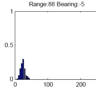
Figure 9b. Noise Histogram for the horizontal FLS at Range 88m and -5 degrees bearing
