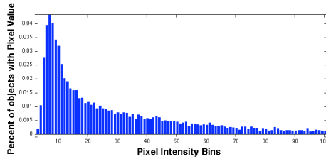
Figure 10. Normalized histogram of pixel intensities from selected objects in horizontal sonar images. Note the graphic has been truncated in the x axis for viewing.
