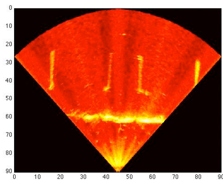
Figure 1. Horizontal Sonar Image – AUV approaches bridge
