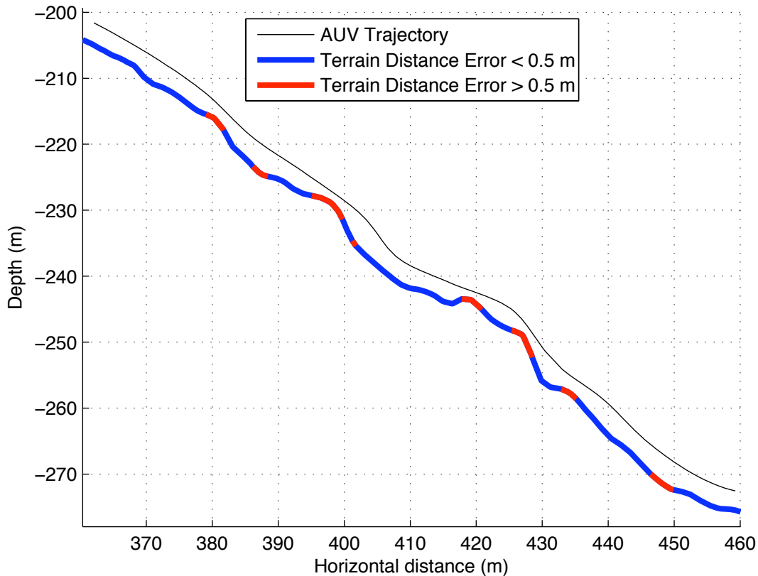
Optimal AUV terrain following trajectory, \rho=10 m
