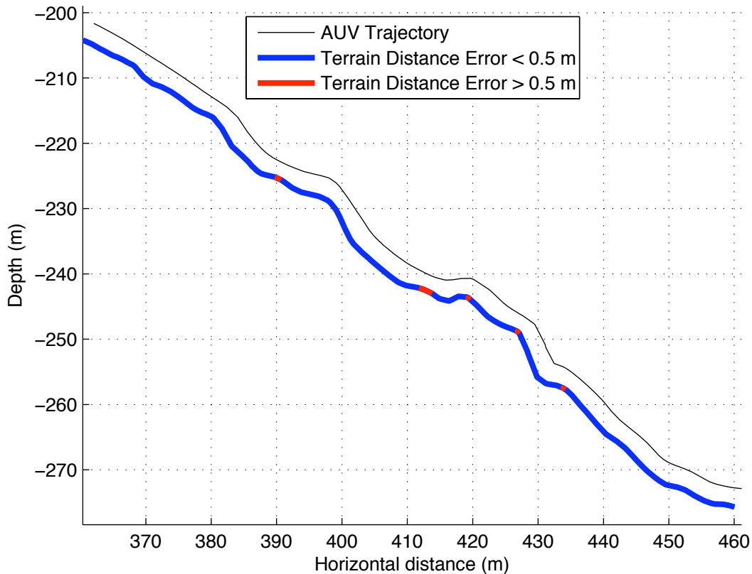
Optimal AUV terrain following trajectory, \rho=4 m
