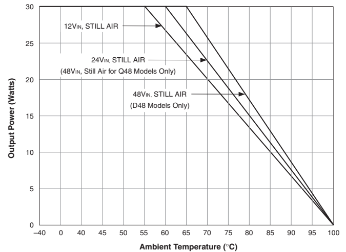
UHE-12/2500 and UHE-15/2000 (All Models) Temperature Derating
