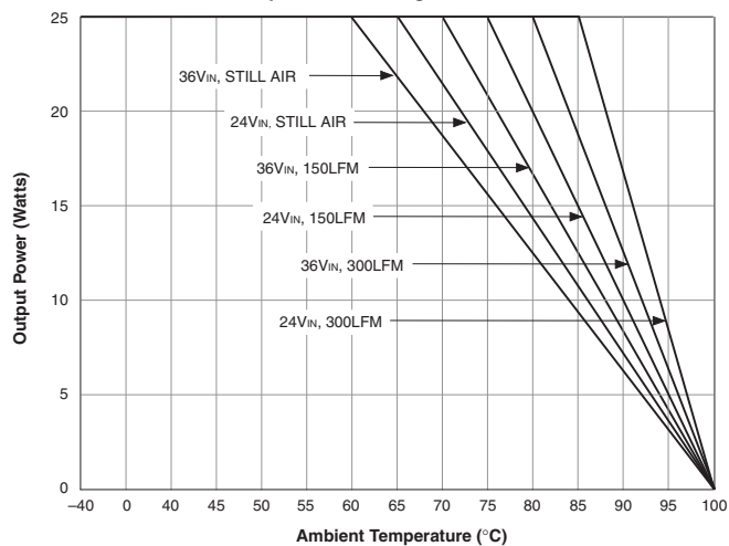
UHE-5/5000-Q12 Temperature Derating
