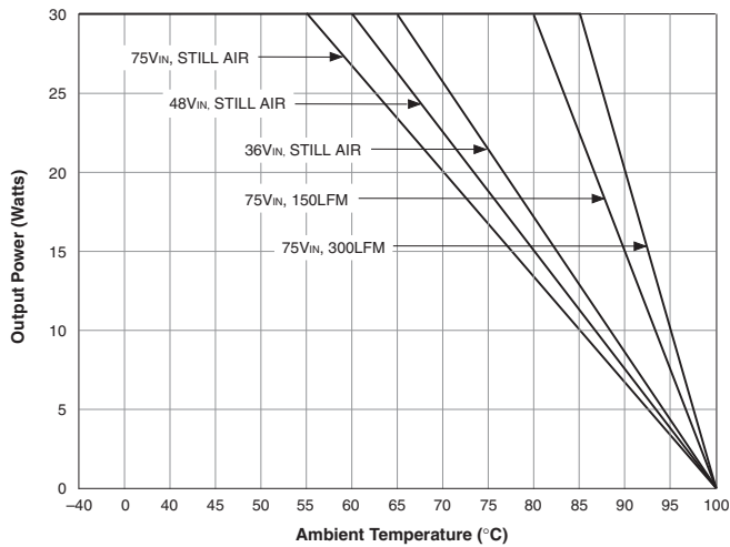
UHE-5/6000-D48 Temperature Derating
