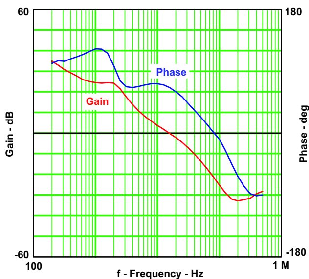
Figure 9. TPS5430 Loop Response
