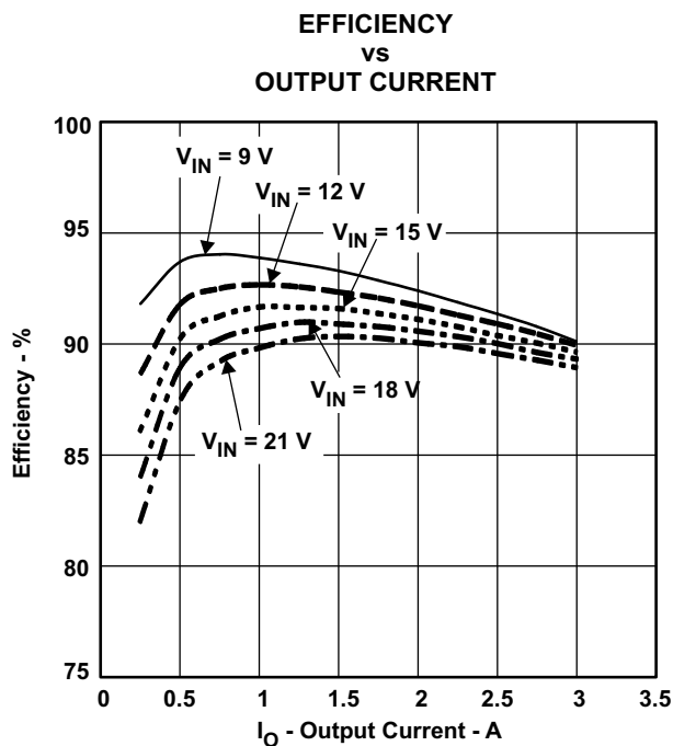
Figure 2. TPS5431 Efficiency
