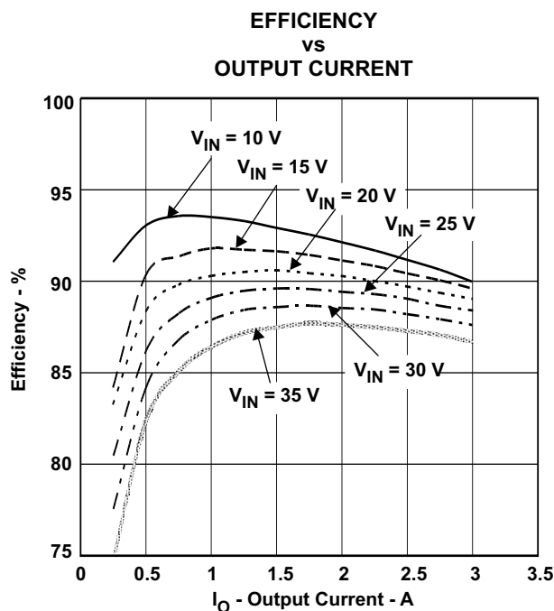
Figure 1. TPS5430 Efficiency
