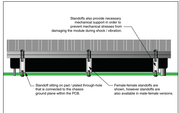
Figure 3-3 — Recommended mounting method using standoffs
